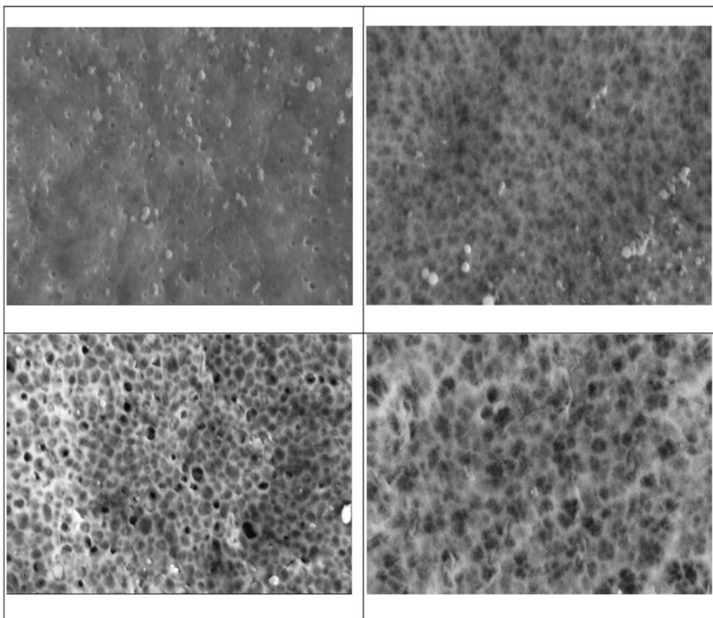
Figure 2: Surface morphology of PVDF-chitosan composite membrane with casting solution composition : (1) 15% PVDF/0,5% chitosan/84% NMP/0,5% \text{NH}_4\text{Cl} ; and (2) 12% PVDF/2% chitosan/84% NMP/2% \text{NH}_4\text{Cl} (stirring temperature 40 °C); (3) 15% PVDF/0,5% chitosan/84% NMP/0,5% \text{NH}_4\text{Cl} ; and (4) 12% PVDF/2% chitosan/84% NMP/2% \text{NH}_4\text{Cl} (stirring temperature 60 °C) (magnification 5000x)
